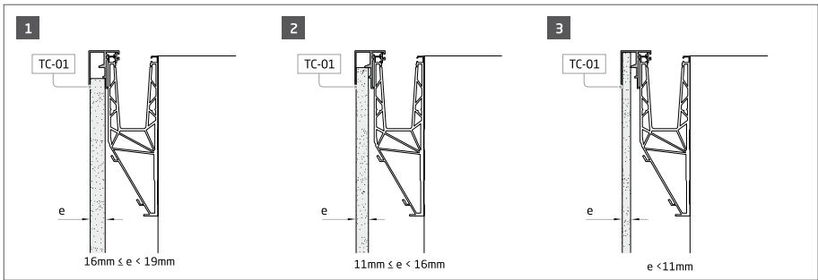
SV-1704 Side Profile Trim TC-01
