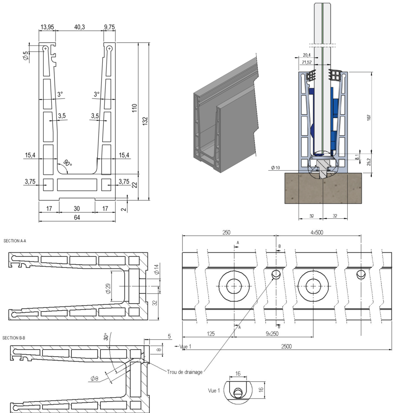
Figure 8 – GlassFit SV-1401 Top – dimensions
