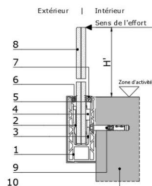
Figure 4 – GlassFit SV-1404 Side – Montage latéral
