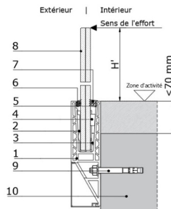
Figure 4 – GlassFit SV-1404 Side – Montage latéral
