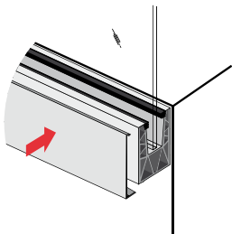
SV-1802 Side Cladding CL-1802-1
