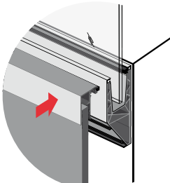
SV-1704 Side Ventilated Rainscreen TC-01
